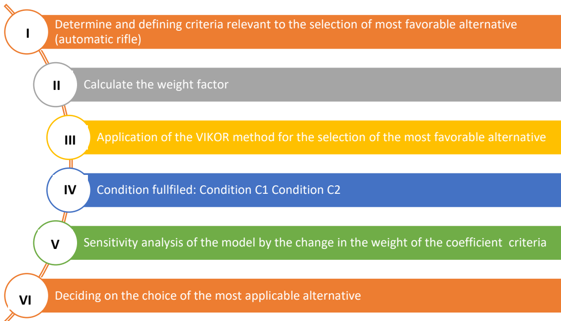
Figure 1. AHP-VIKOR model
